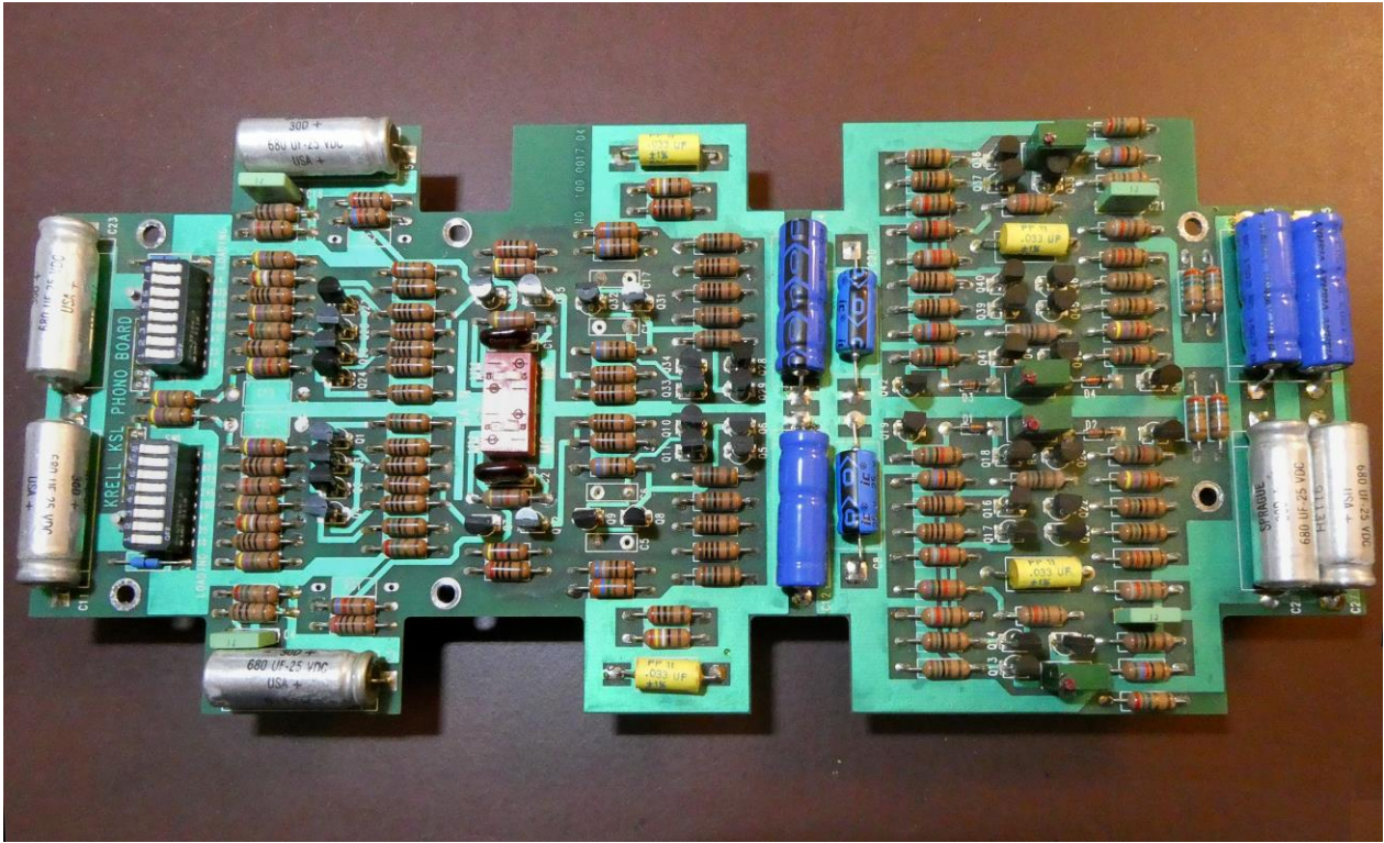
Phono Board
